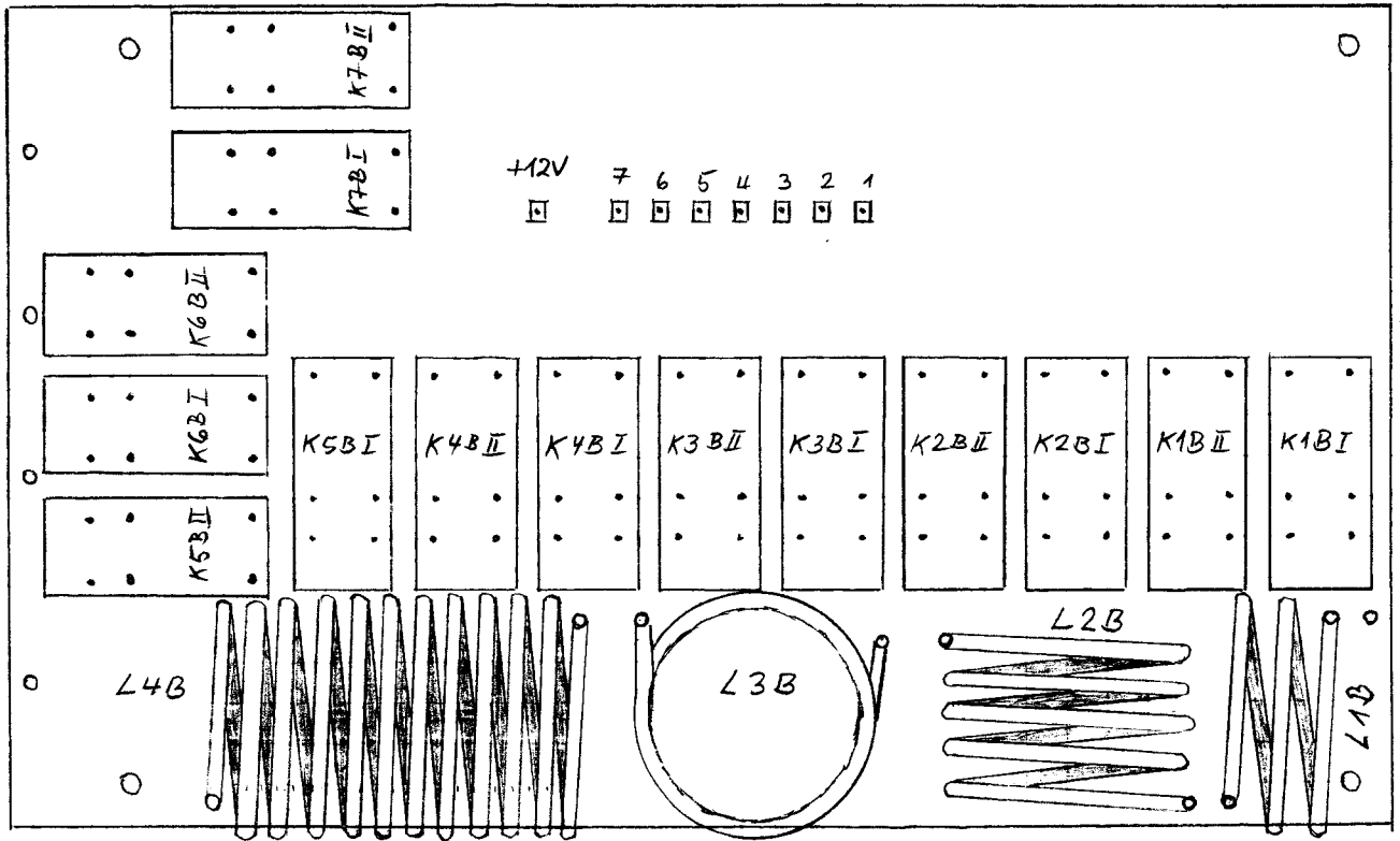
Spulenplatine B
