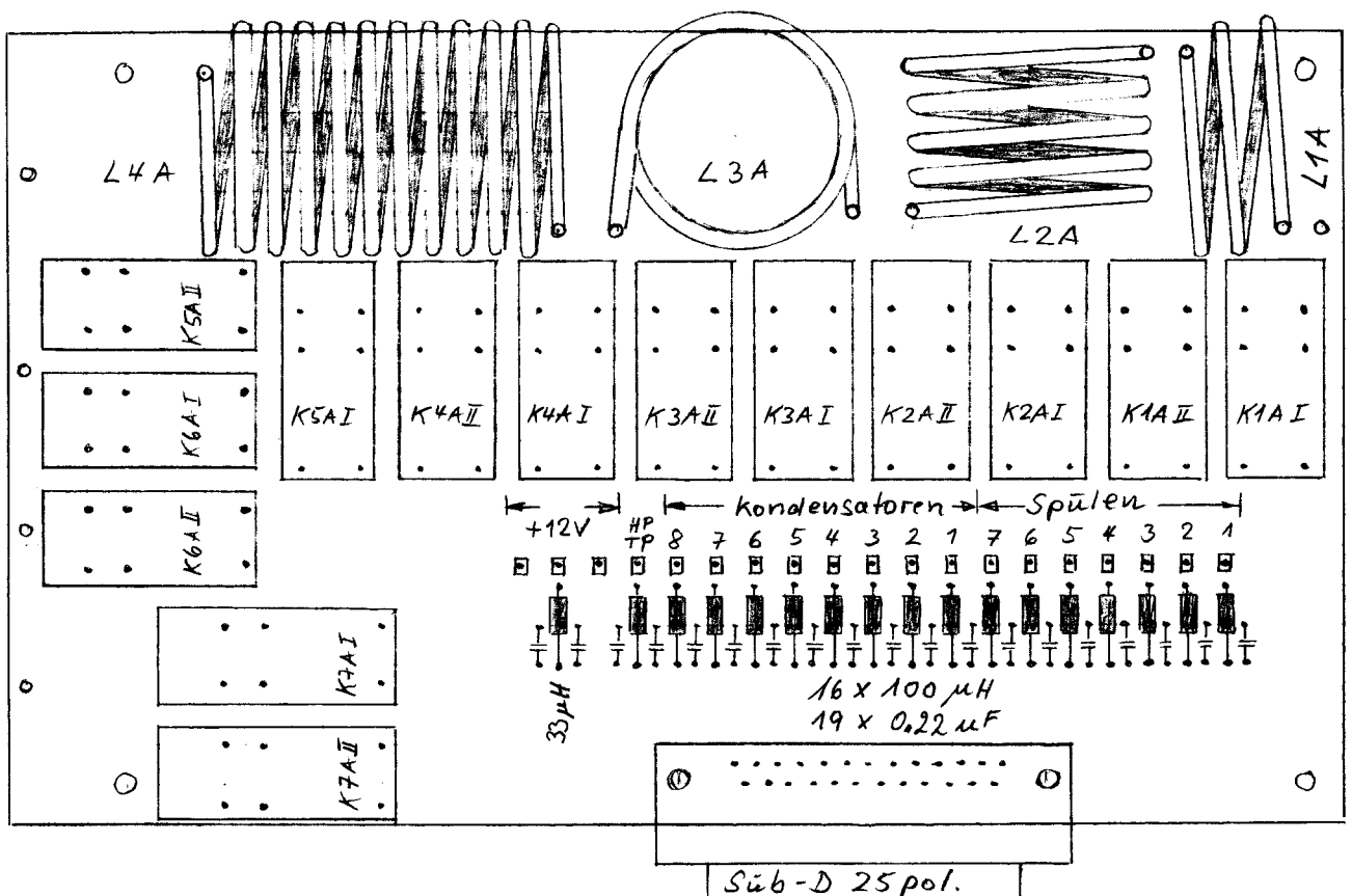
Spulenplatine A
